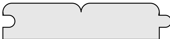
KW # 074 3/4" x 3-1/4" FACE
