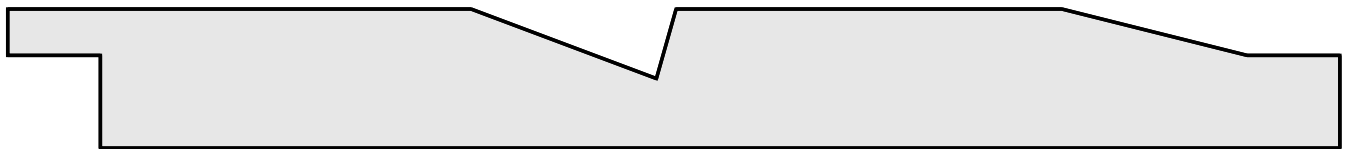
KW # 600 3/4" x 6-3/4" FACE-7-3/16" O.A.
