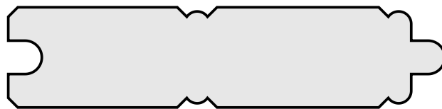
KW # 1039 3/4" x 3" FACE
