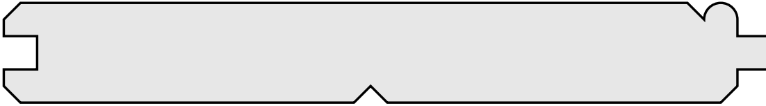
KW # 2939 3/4" x 5-1/2" FACE
