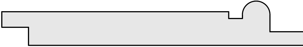
KW # 2106 13/16" x 4-7/8" FACE - 5-1/2" O.A.
