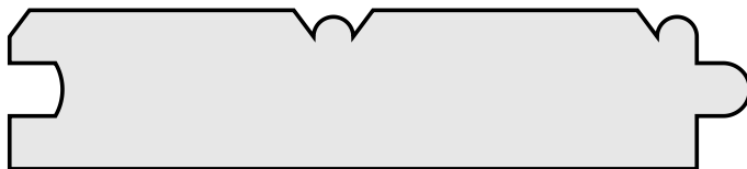
KW # 3265 3/4" x 3-1/4" FACE
