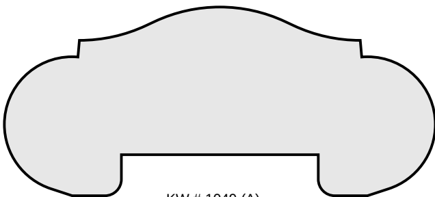
KW # 1049 (A) 1-7/16" x 3-1/4"
