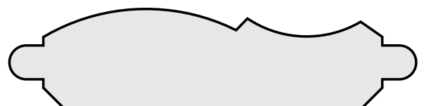
KW # 2375 3/4" x 2-1/2" FACE - 3 O.A.
