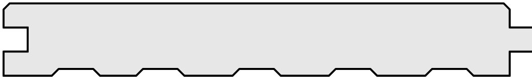
KW # 740 3/4" x up to 11" Face
