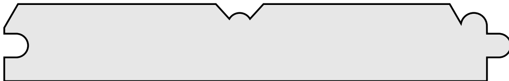
KW # 116 13/16" x 5-1/16" Face
