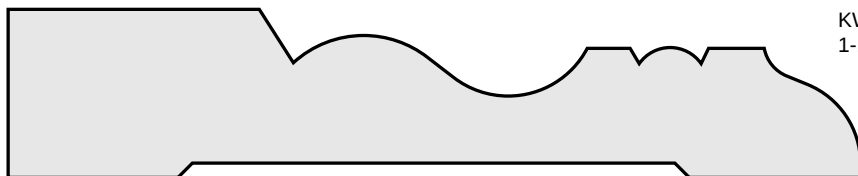
KW # 1863 (A) 7/8" x 4-7/16"
