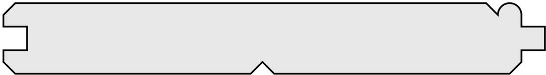
KW # 2939 3/4" x up to 11" FACE
