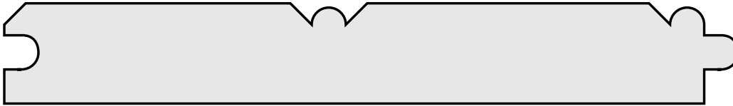
KW # 2968 3/4" x 5-1/8" FACE
