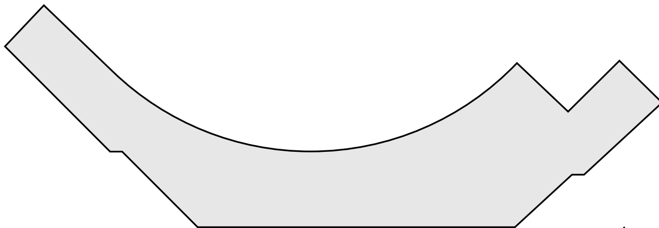
KW # 2521 2-1/4" x 6-3/4"
