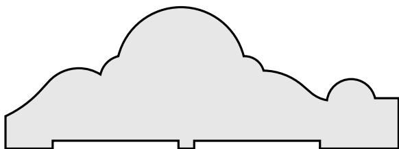
KW # 1339 (A) 1-1/8" x 3-1/8"
