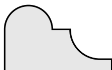
KW # 3133 11/16" x 1-1/8"
