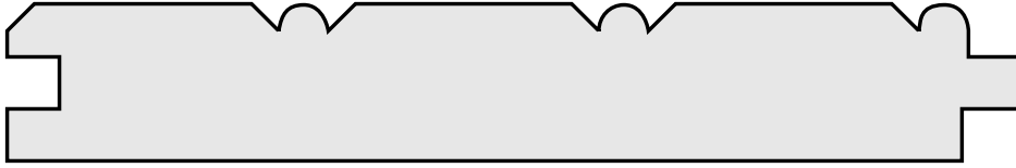
KW # 2858 3/4" x 4-19/32" FACE
