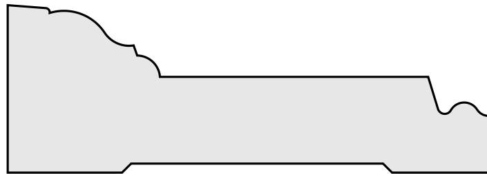
KW # 2409 1-5/16" x 3-3/4"
