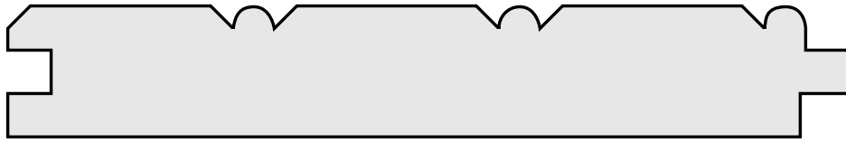
KW # 2858 3/4" x 4-19/32" FACE
