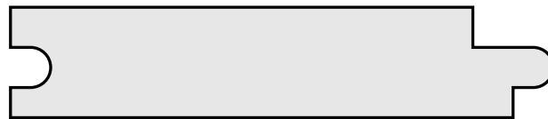
KW # 2923 11/16" x up to 11" FACE
