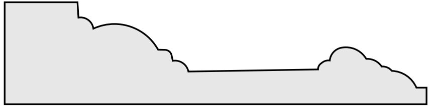
KW # 2199 1-1/16" x 4-3/8"
