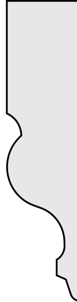
KW # 900 3/4" x 3"
