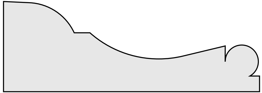
KW # 2005 1-1/2" x 4-1/4"
