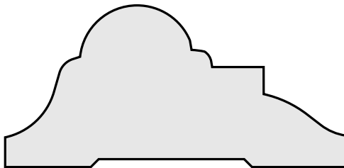
KW # 365 1-3/16" x 2-1/2"
