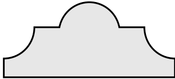
KW # 2692 3/4" x 1-3/4"
