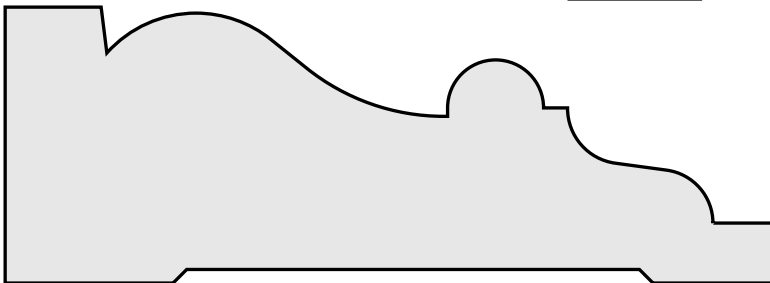
KW # 3160 1-7/16" x 4"
